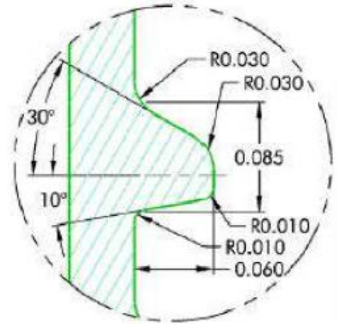
GLASS THREAD DETAIL SCALE 10 : 1
