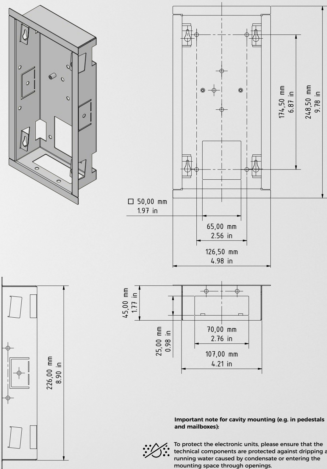
D2101V Flush-mounting housing (backbox)
