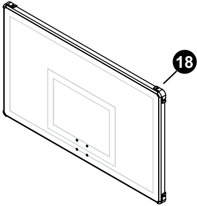
BACKBOARD ASSEMBLY, 60" x34" 4A-8677-20 QTY. 1
