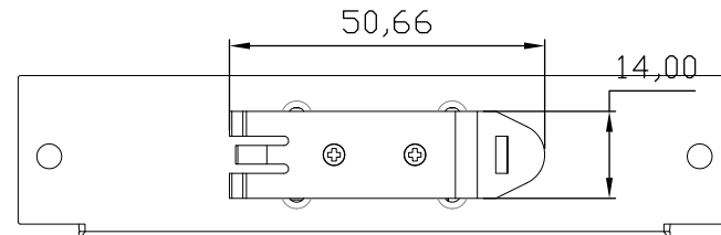
clip detail
