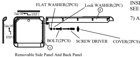
Removable Side Panel And Back Panel
