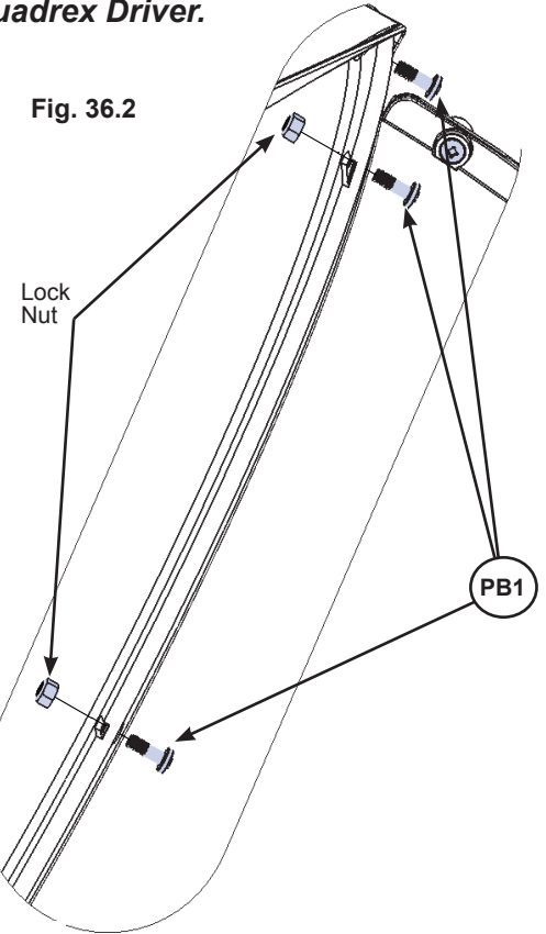
Bottom of Slide Views
