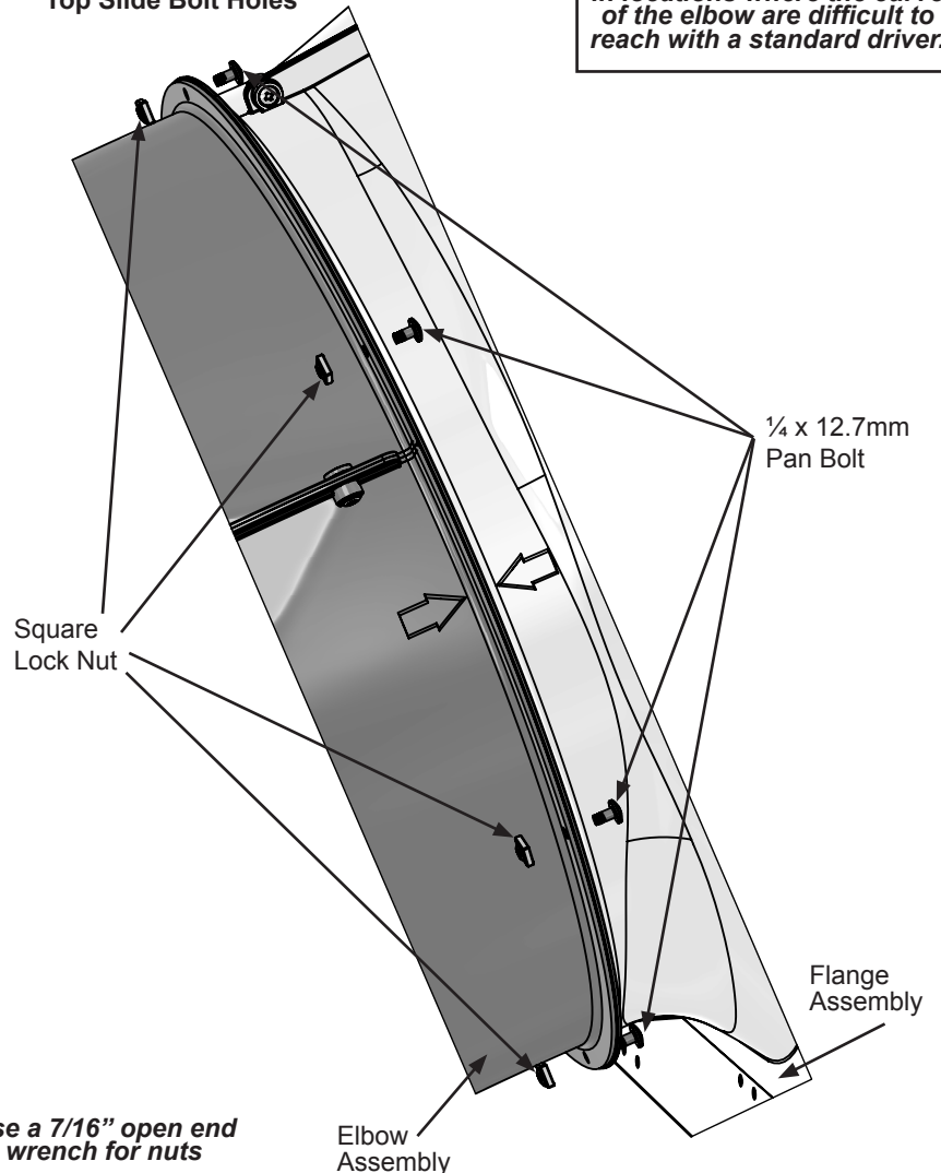
Fig. 35.2 Top Slide Bolt Holes
