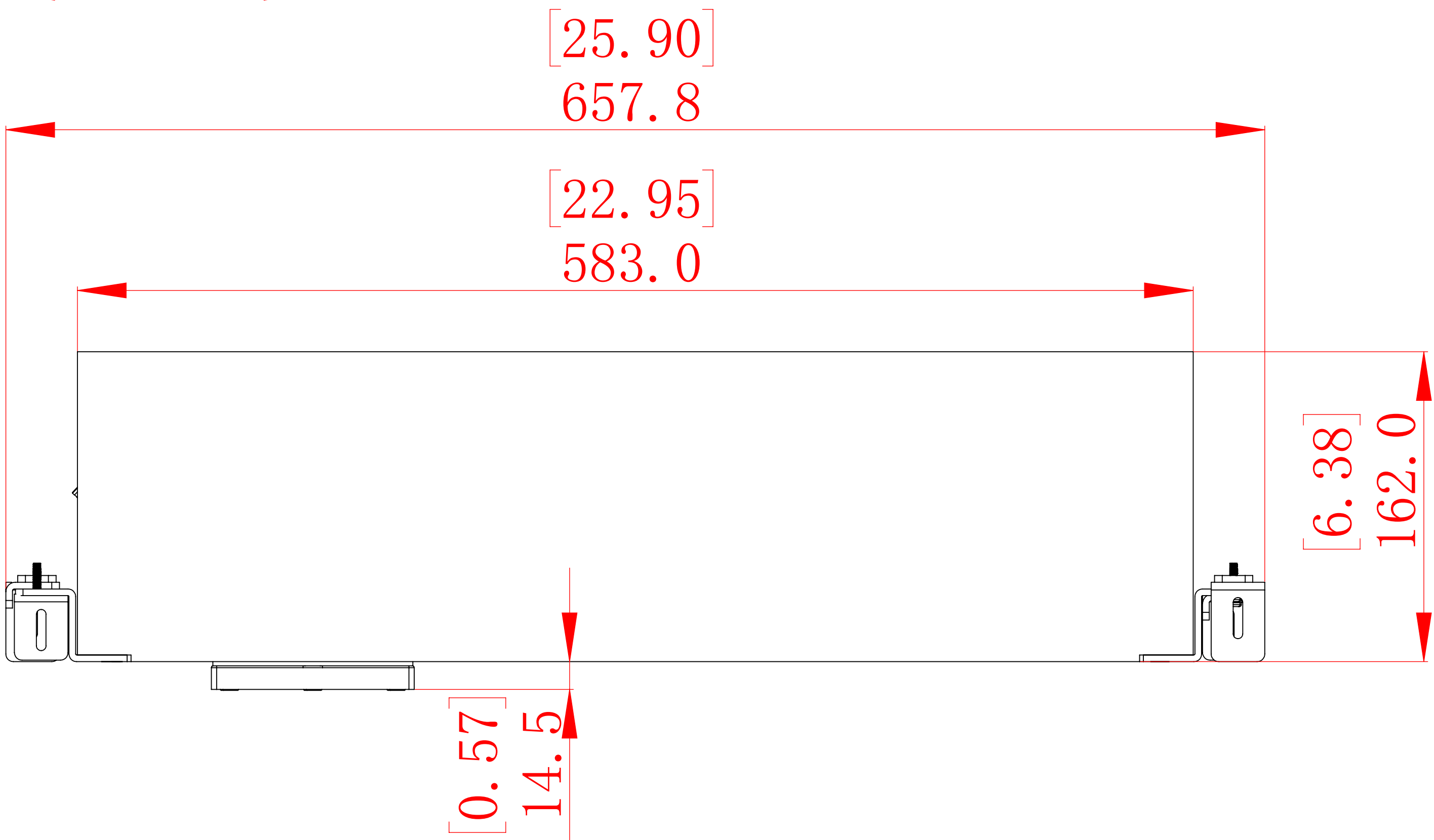
SIDE VIEW
