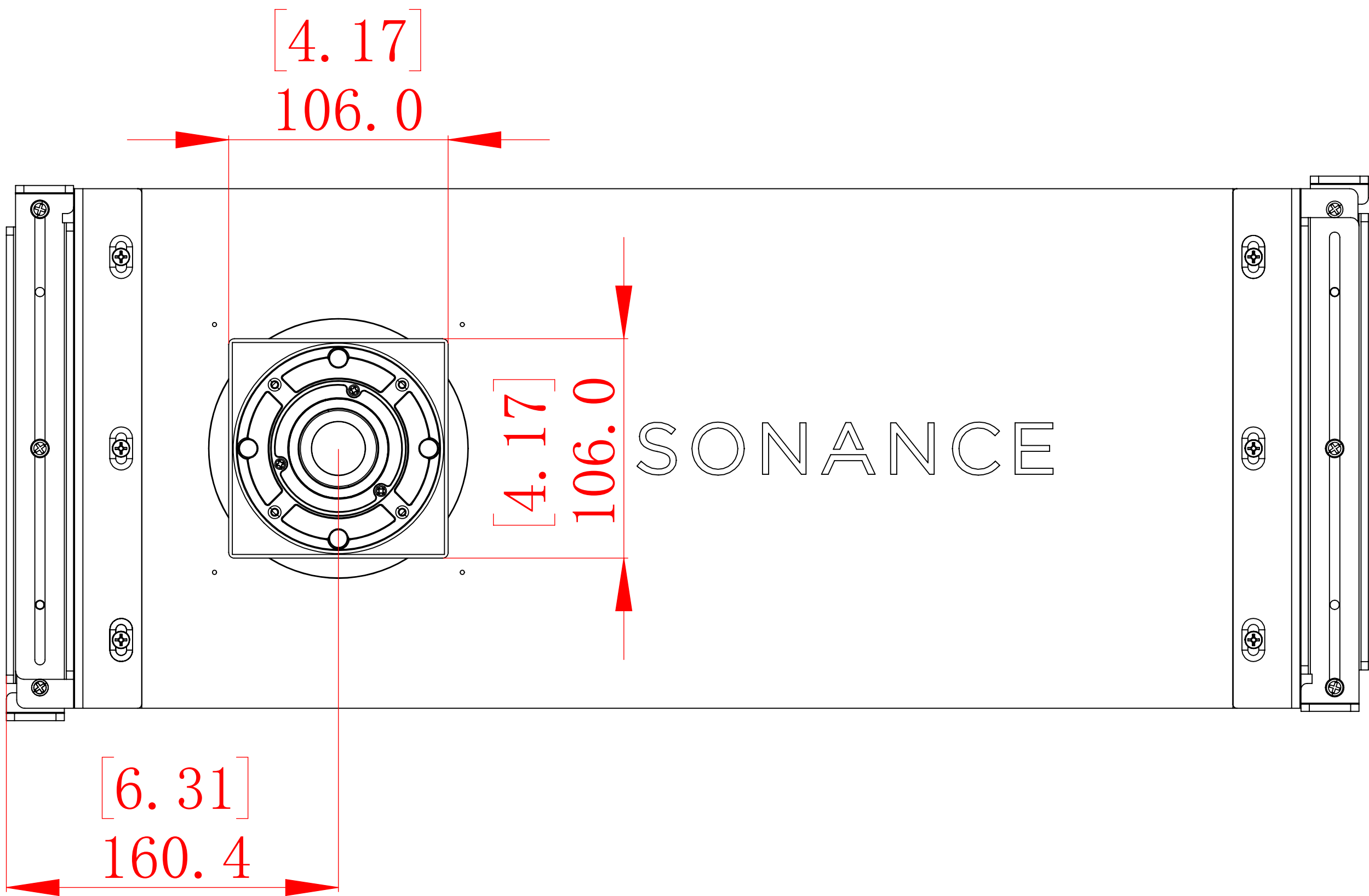
FRONT VIEW
