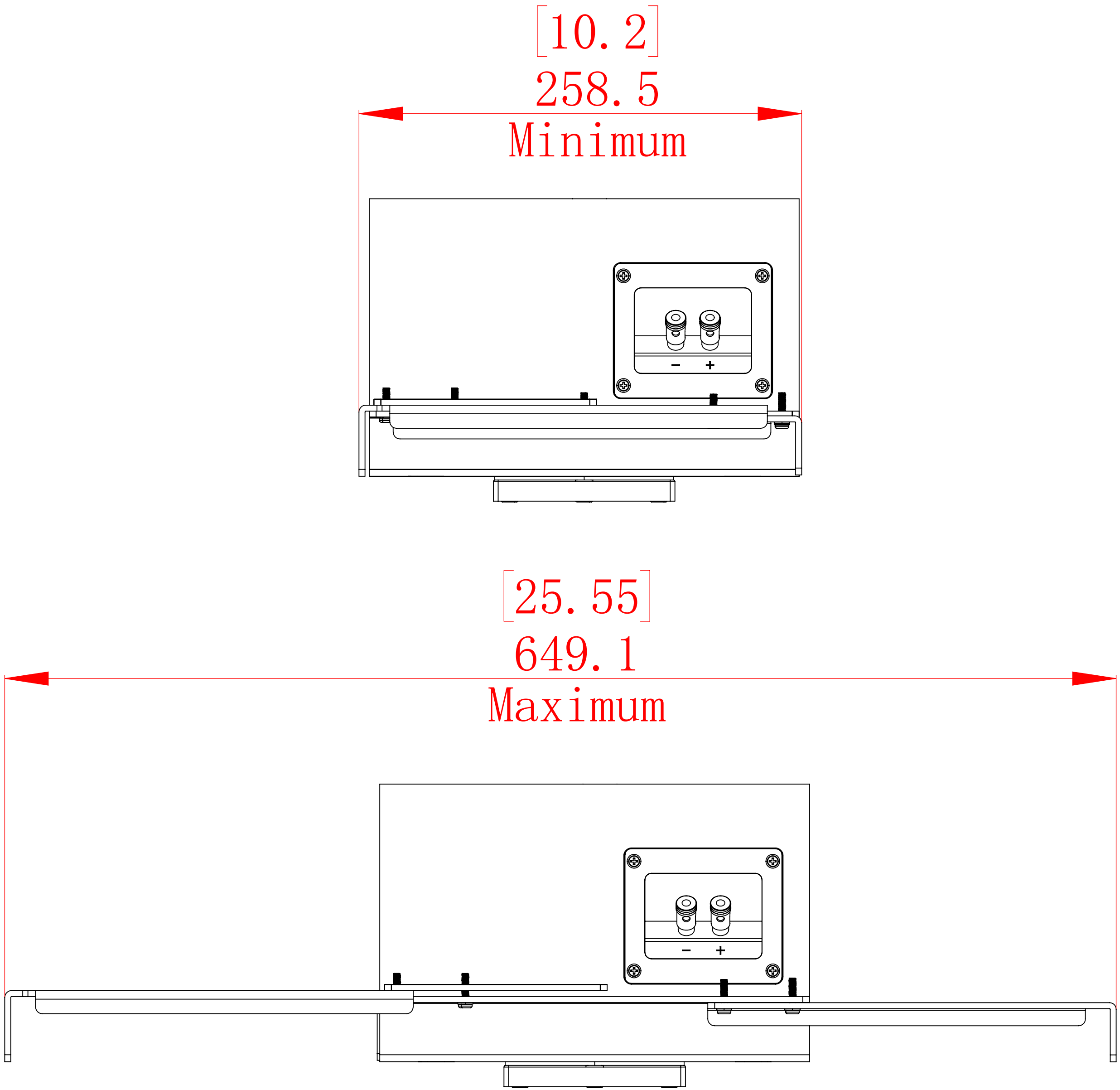
SIDE VIEW
