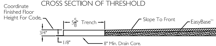
CROSS SECTION OF THRESHOLD
