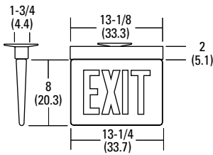
Top Mount (AC only operation)
