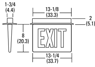
Ceiling Mount (recessed)
