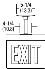
With Pendant Mounting kit (TM mounting only)
