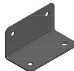
A100140 (2) | SUPPORT EN L 66x66x127
