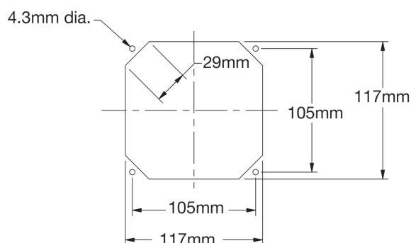
Mounting hole dimensions for QFAN-119, FAN-119, AXS-FAN-119
