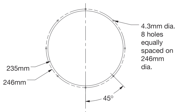
Mounting hole dimensions for FAN-254
