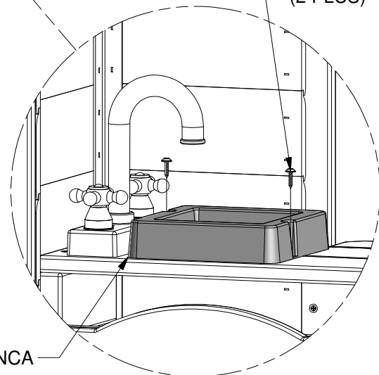
TORNILLO PWH #8 x 5/8" (2 PLCS)
