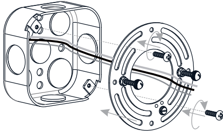
(2) Alternative Screws
