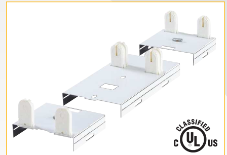
8-FT T8 RETROFIT KIT - P/N 14050
