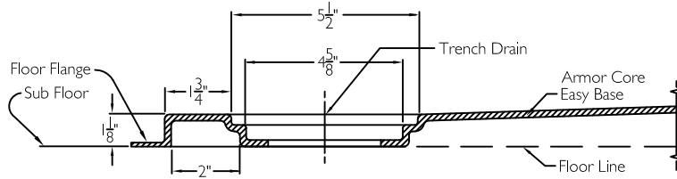
CROSS SECTION OF SHOWER BASE
