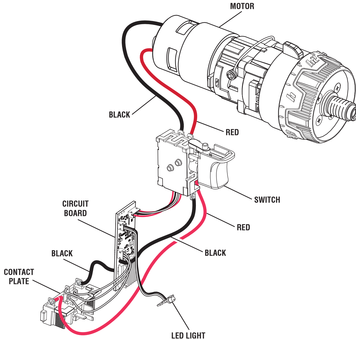
WIRING DIAGRAM
