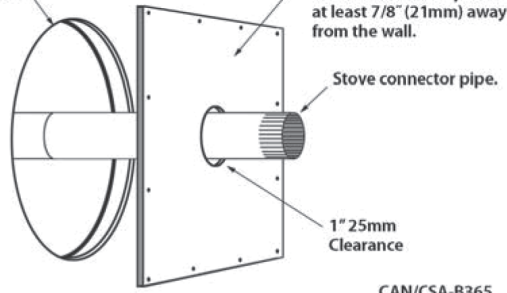
Figure 4 ONLY APPROVED CANADIAN WALL PASS THROUGH
