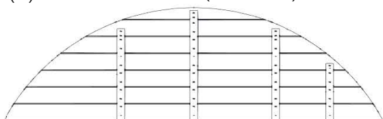
WP03 ASSEMBLAGE DE PANNEAU MURAL-W2A04786 (x1) 1 3/8"x20 1/8"x66 1/4" (35x512x1199)
