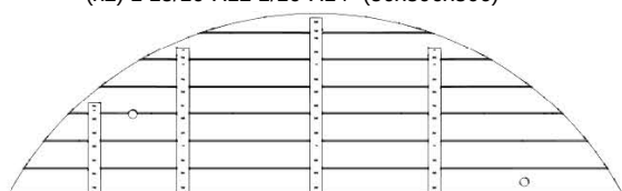
WP01 ASSEMBLAGE DE PANNEAU MURAL - W2A04784 (x1) 1 3/8"x19 11/16"x65 3/4" (35x500x1169)
