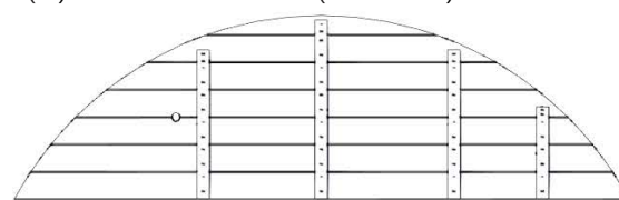
WP06 ASSEMBLAGE DE PANNEAU MURAL - W2A04809 (x1) 1 3/8"x20 1/8"x66 1/4" (35x512x1491)
