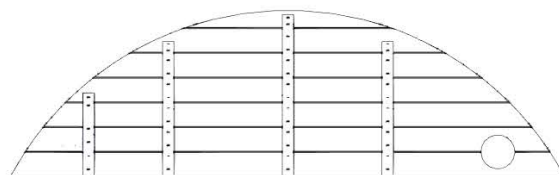
WP05 PANNEAU MURAL - W2A04792 (x1) 1 3/8"x19 11/16"x65 3/4" (35x500x1337)
