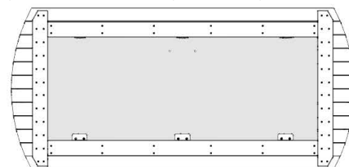
WP04 ASSEMBLAGE DE PANNEAU MURAL - W2A04794 (x1) 2 3/8"x35 5/8"x74 9/16" (60x906x201)
