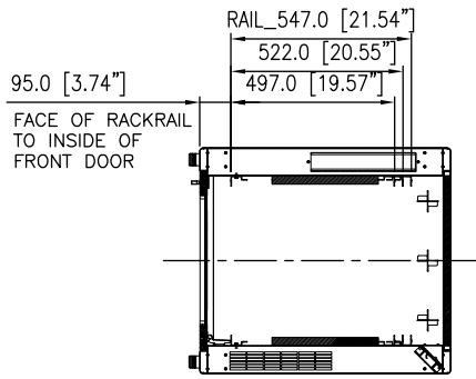
SECTION A-A FRONT RAIL ADJUSTABLE TO 95 [3.74"], 120 [4.7"], AND 145 [5.7"] FROM INSIDE OF FRONT DOOR
