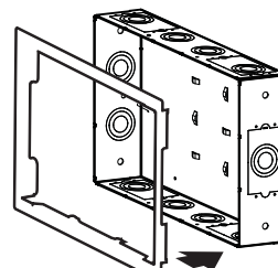
C - Reinstall box flange. Reattach screws.
