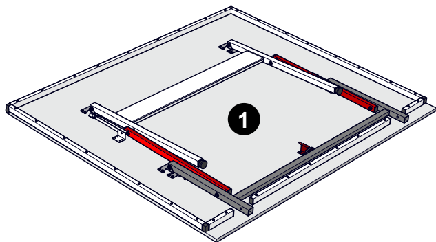
PRE-ASSEMBLED TABLE TOP 4A-6603-03 (QTY. 2)
