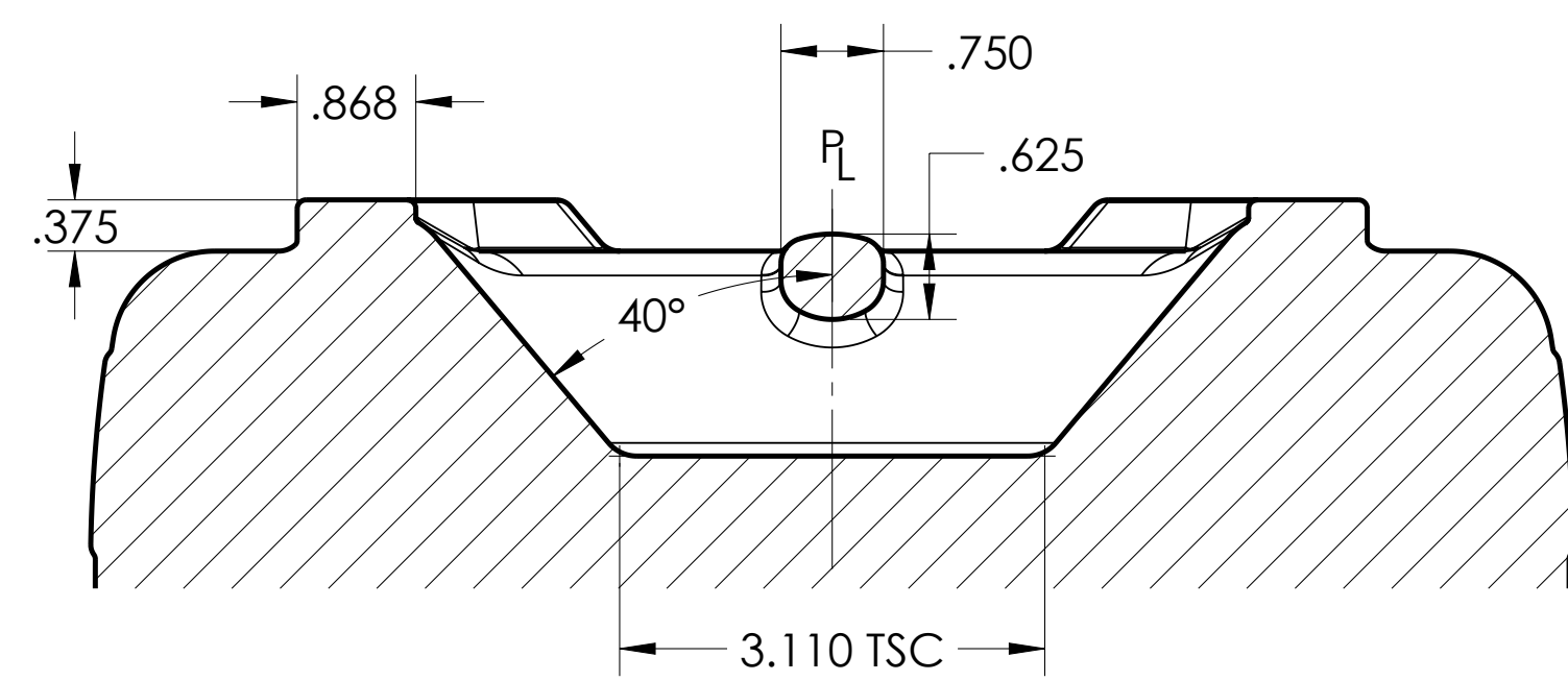
SECTION B-B
