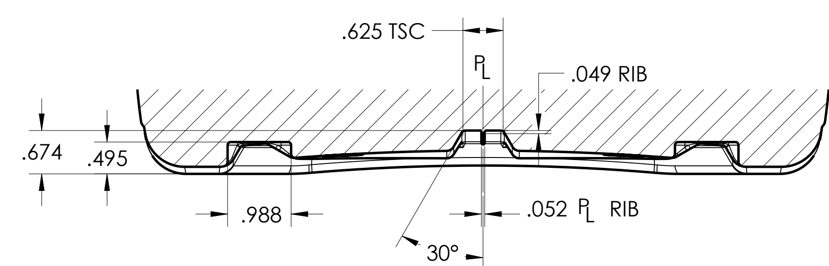
SECTION C-C
