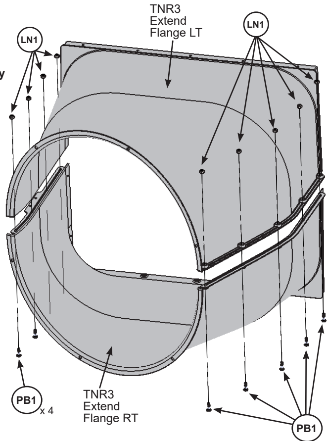
Fig. 73.2 Flange Assembly
