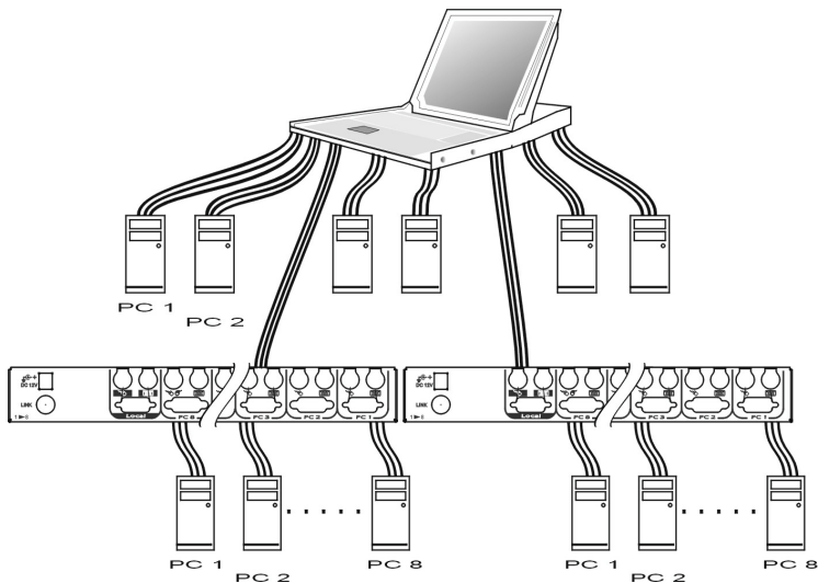
Figure 2: A cascaded KVM Module configuration
