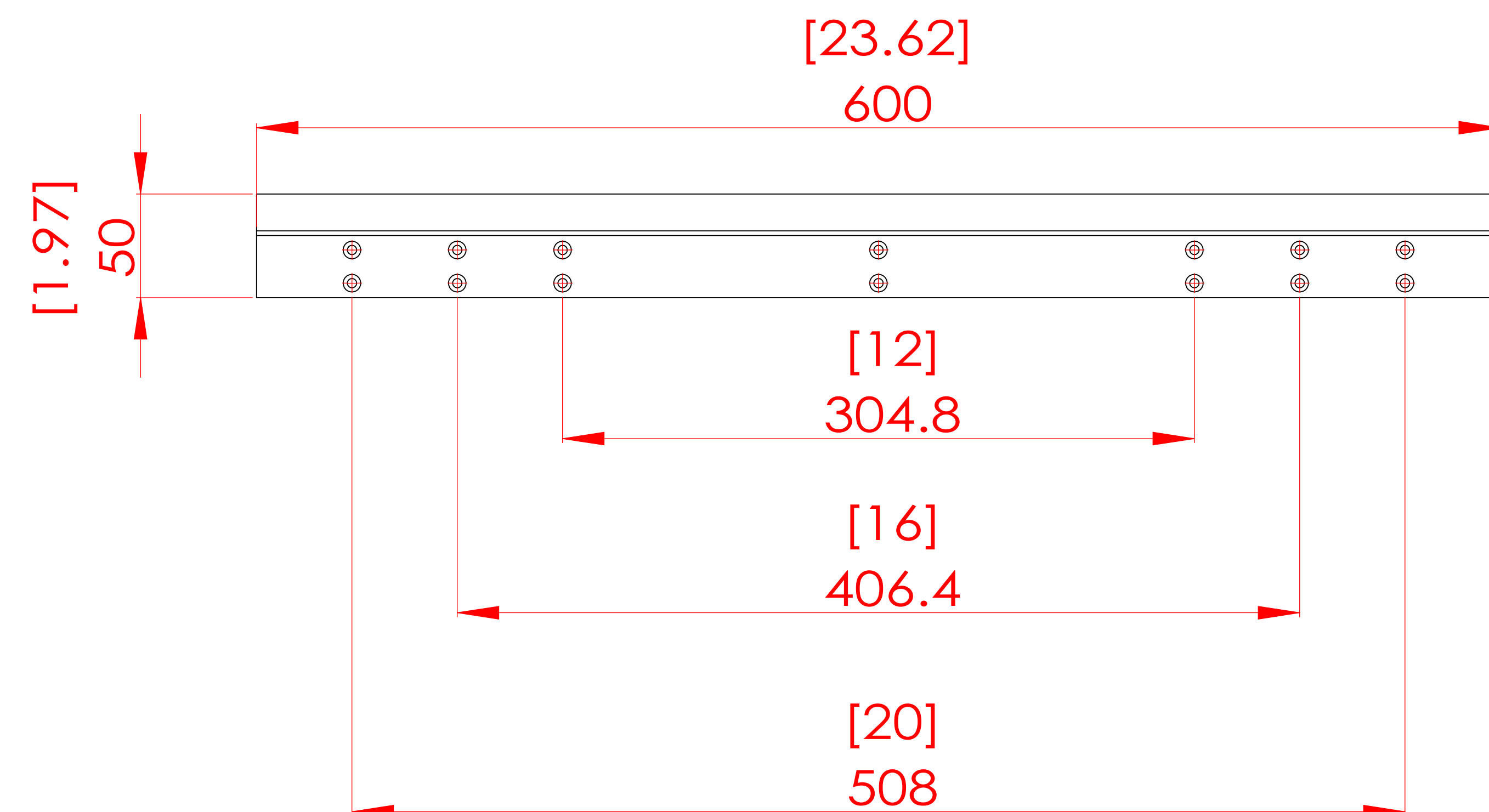
WALL Z-CLIP
