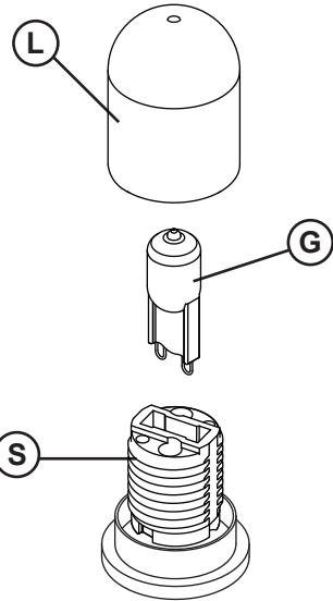
Drawing 2 - LED
