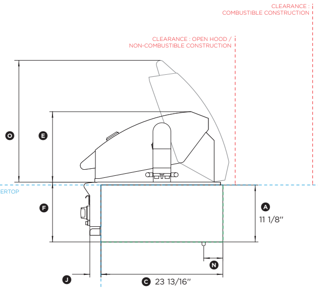
PROFILE VIEW
