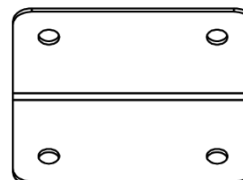
A100140 | SUPPORT EN L (x2) 66 x 66 x 127
