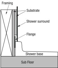
Flange Details: Fire Rated Walls (U.S.) Flange Details: (U.S.)
