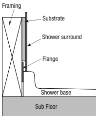
Flange Details: Fire Rated Walls (U.S.) Flange Details: (U.S.)
