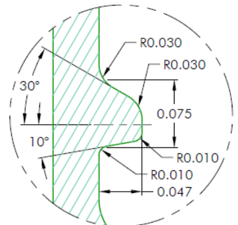
PLASTIC THREAD DETAIL SCALE TO : 1
