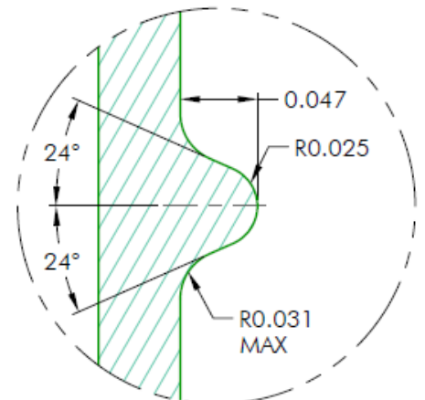
GLASS THREAD DETAIL SCALE TO : 1
