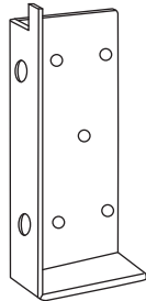
D. Right bracket D. Support droit
