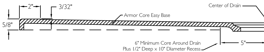
CROSS SECTION OF THRESHOLD
