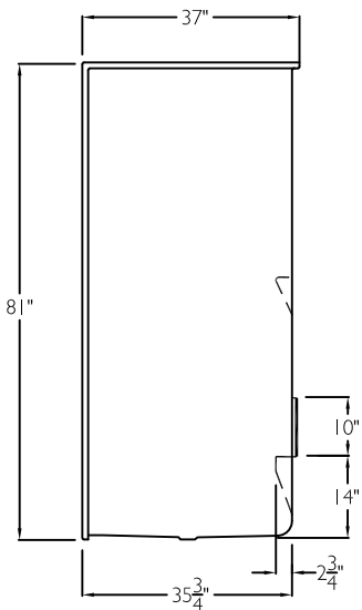
CROSS SECTION OF THRESHOLD
