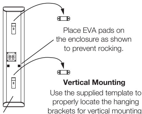
Fig. 4 Wall Mounting
