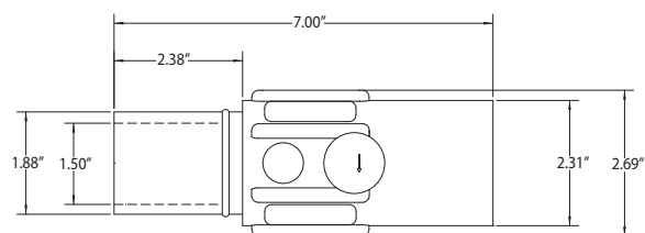
Male Connector
