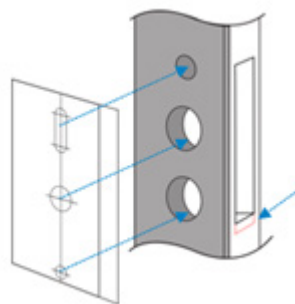
Step 2 Chisel/file mortice pocket as per template.
