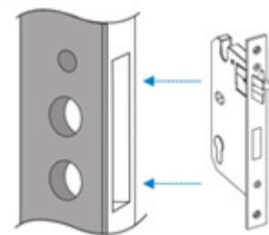
Step 3 Install Schlage Resolute mortice lock and assemblies.
