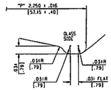
STACKER DETAIL SCALE 10 TO 1
