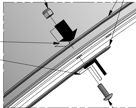
148 (x12) NUT - 1/4"
