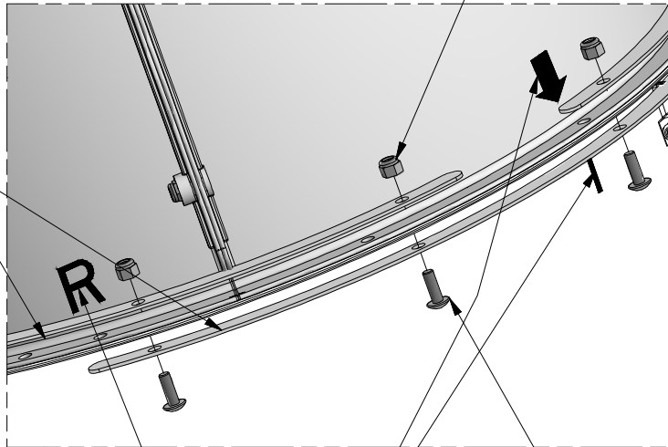
148 (x12) NUT - 1/4"
