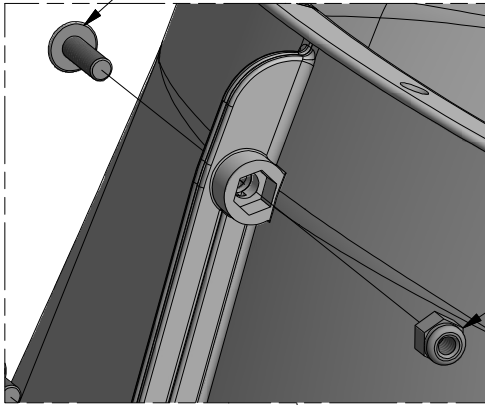
769 (x8) BOLT - 3/4"
