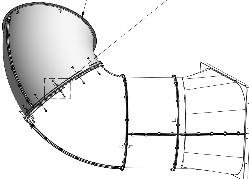
ELBOW TUBE SUB-ASSEMBLY
