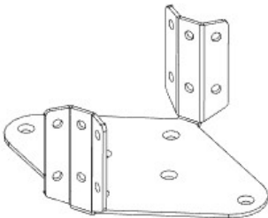
A4M02501 (x1) | FAN MOUNTING BRACKET
