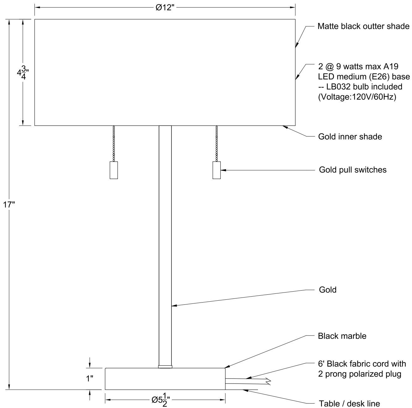
FRONT VIEW
