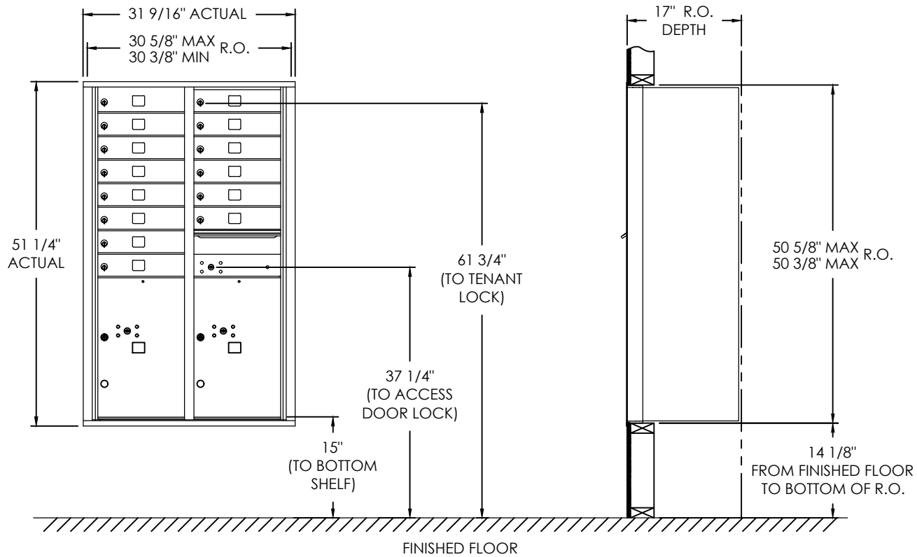
COMPARTMENT CHART
