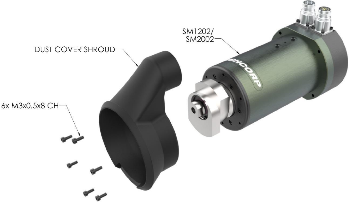
FIGURE 6: DUST SHROUD INSTALLATION STEP 2
