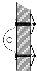
FIGURE B DRYWALL W/O STUDS
