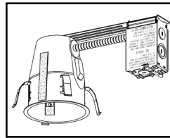
3" Housing
