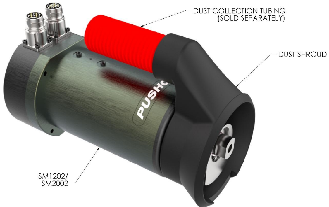
FIGURE 8: DUST COLLECTION SETUP
