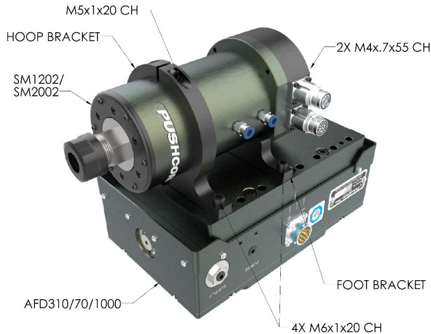
FIGURE 1: PARALLEL MOUNT
