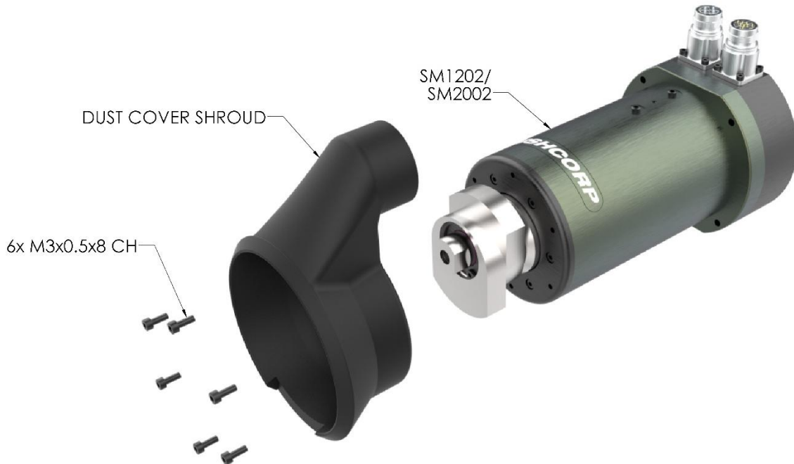
FIGURE 6: DUST SHROUD INSTALLATION STEP 2
