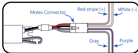
(C) Connect DC output using 4-way connector.
