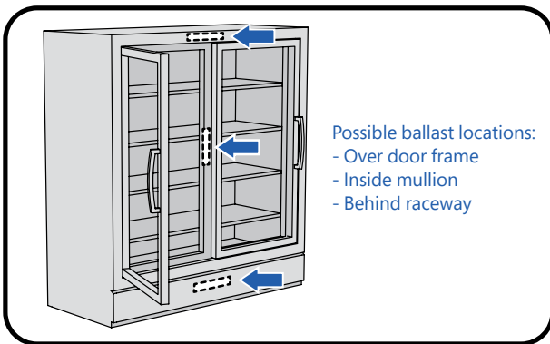
4 Locate ballast and remove access cover. NOTE: Refer to the refrigeration manual for specific ballast location.
