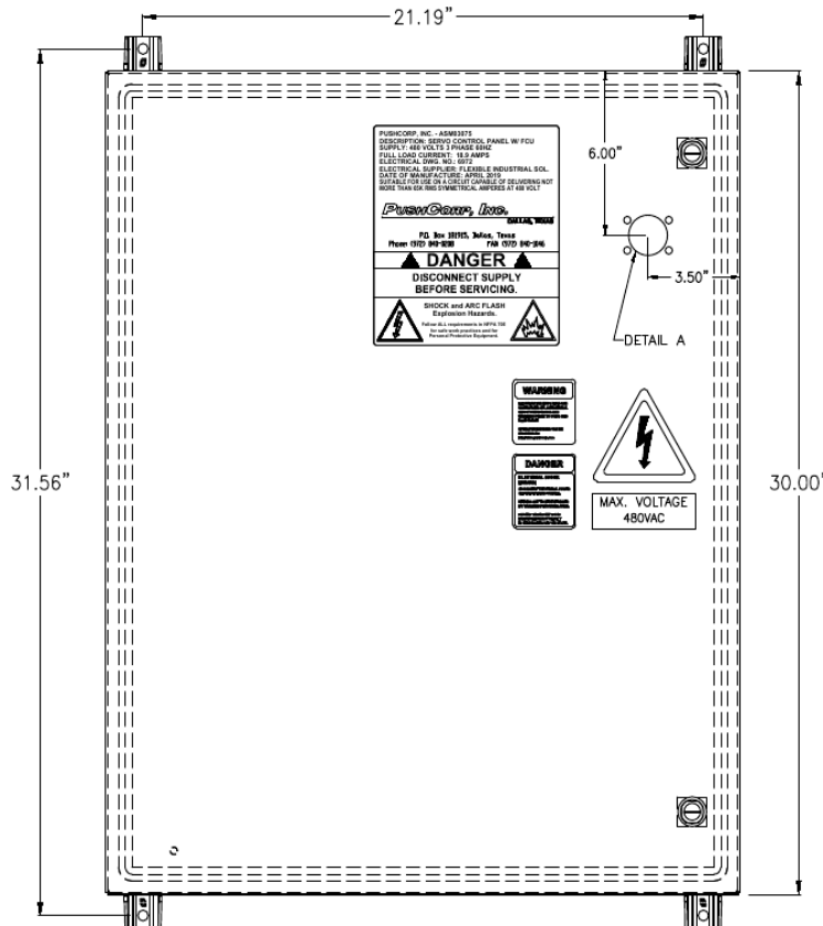
Figure 1: Cabinet Mounting
