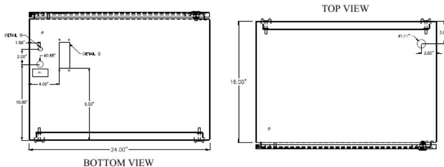
Figure 2: Panel Entry Locations
