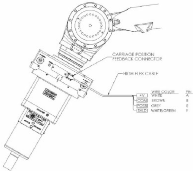
Figure 4: External IO Connections
