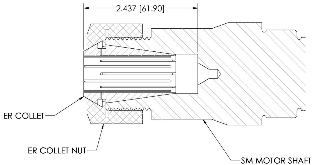
FIGURE 7: SM0612 COLLET DRAWING
