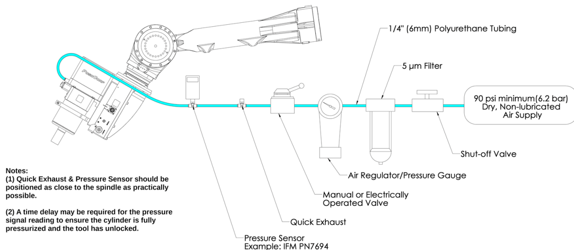
FIGURE 12: PNEUMATIC CONNECTIONS
