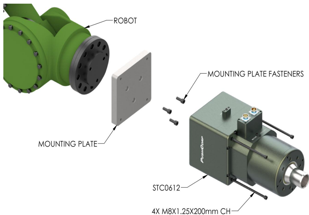
FIGURE 4: STC0612 DIRECT MOUNTING
