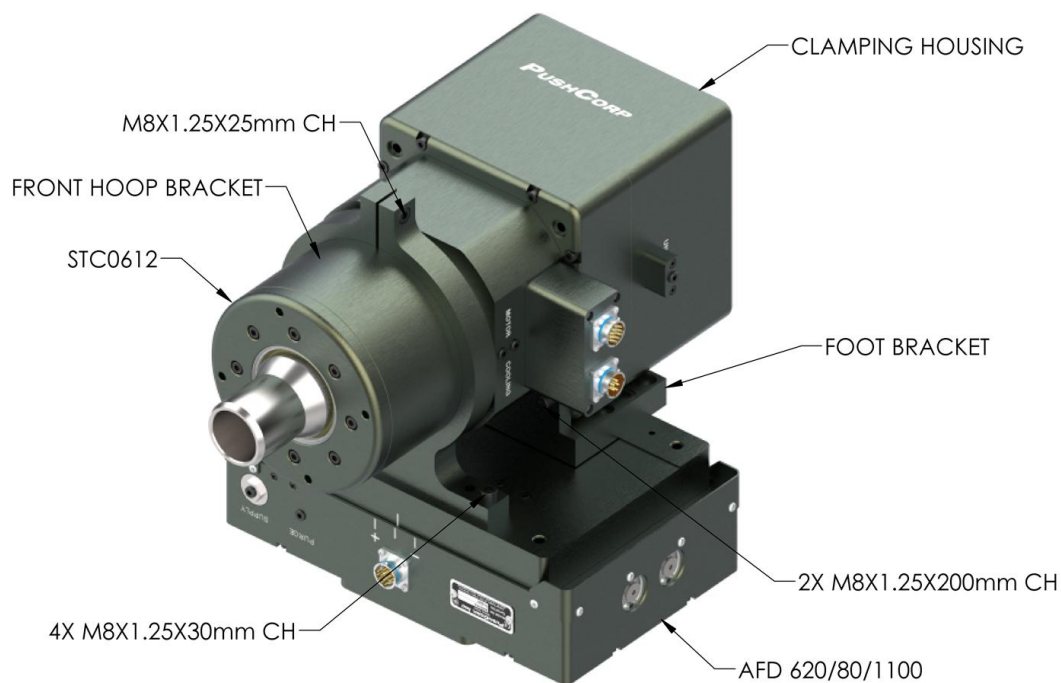
FIGURE 2: 0612-CROSS-AXIS-CONFIGURATION
