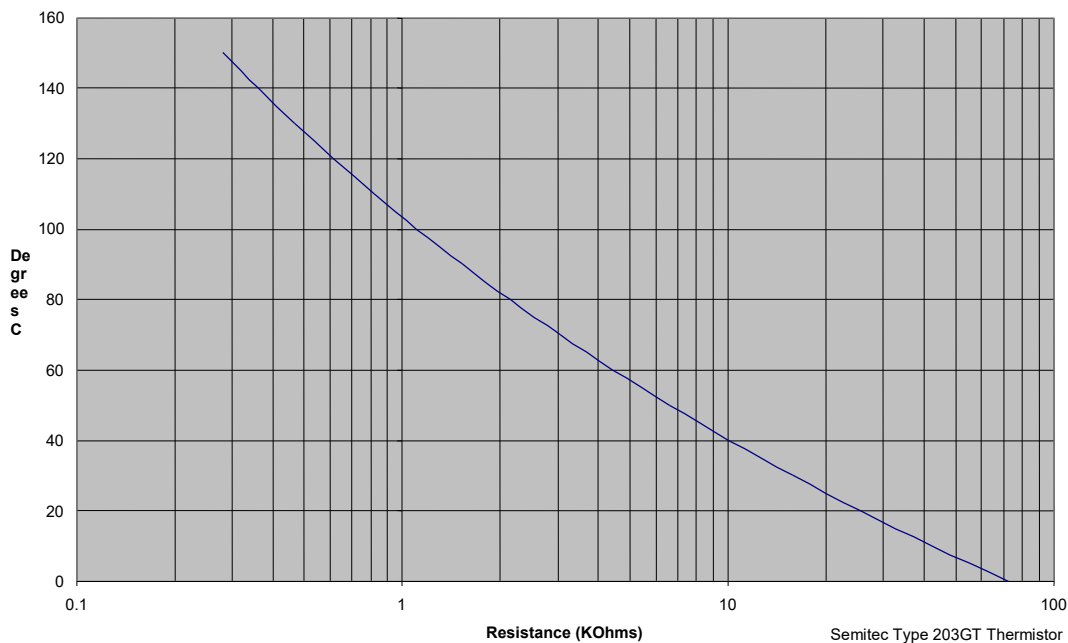
FIGURE 17: THERMISTOR CHART
