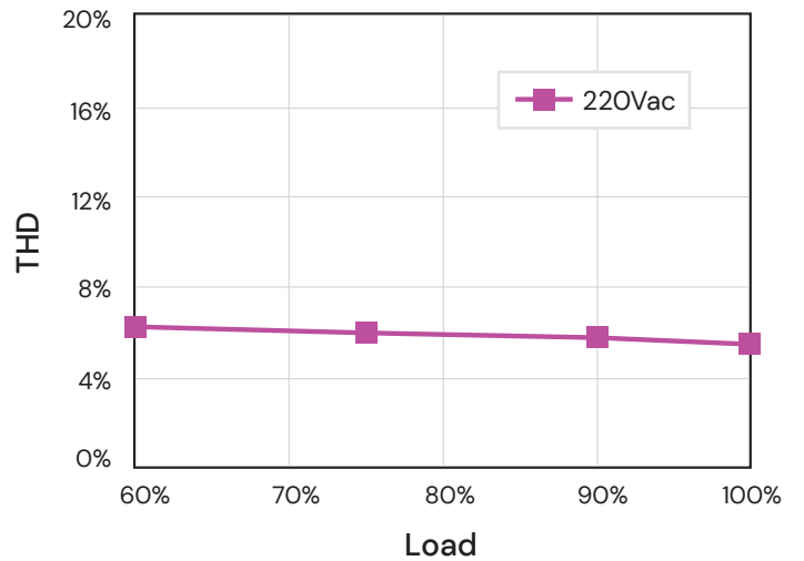
Total Harmonic Distortion
