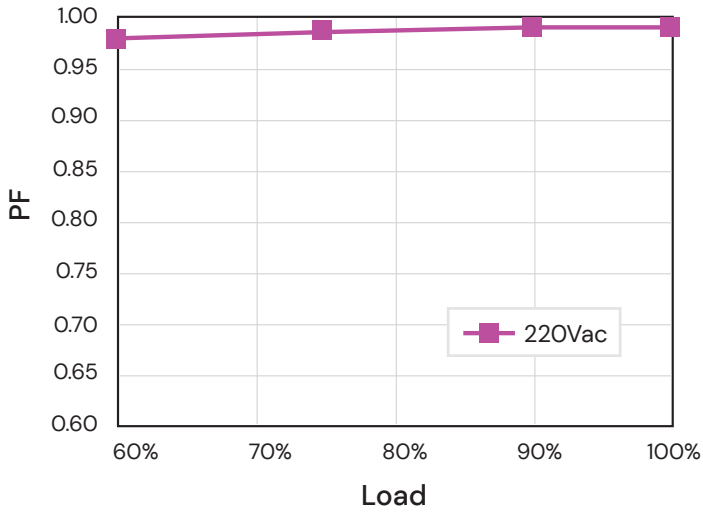
Power Factor
