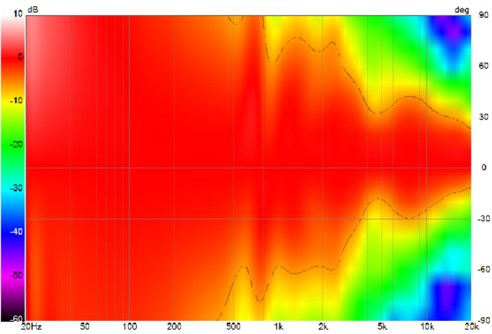
HORN DIRECTIVITY | HORIZONTAL
