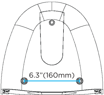
Loudspeaker Top
