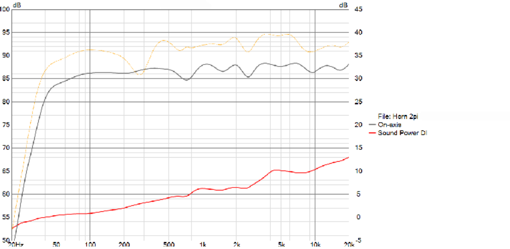
HORN SPL
