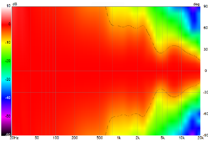
HORN DIRECTIVITY | VERTICAL
