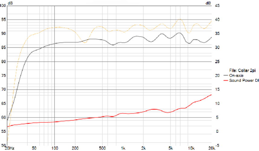
COLLAR SPL
