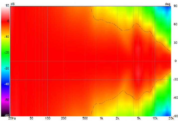
COLLAR DIRECTIVITY | VERTICAL
