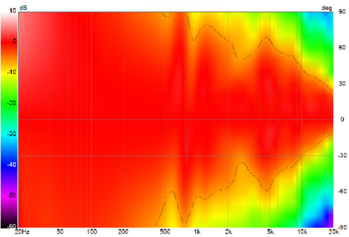
COLLAR DIRECTIVITY | HORIZONTAL
