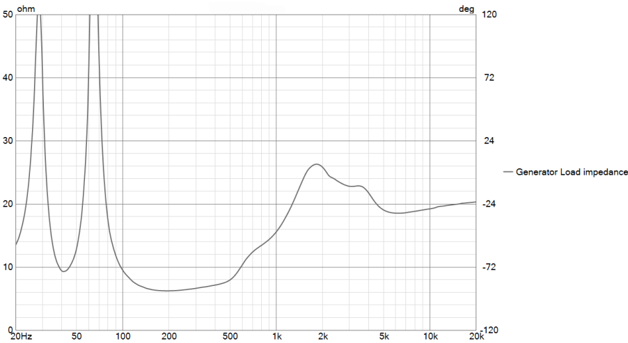
HORN IMPEDANCE
