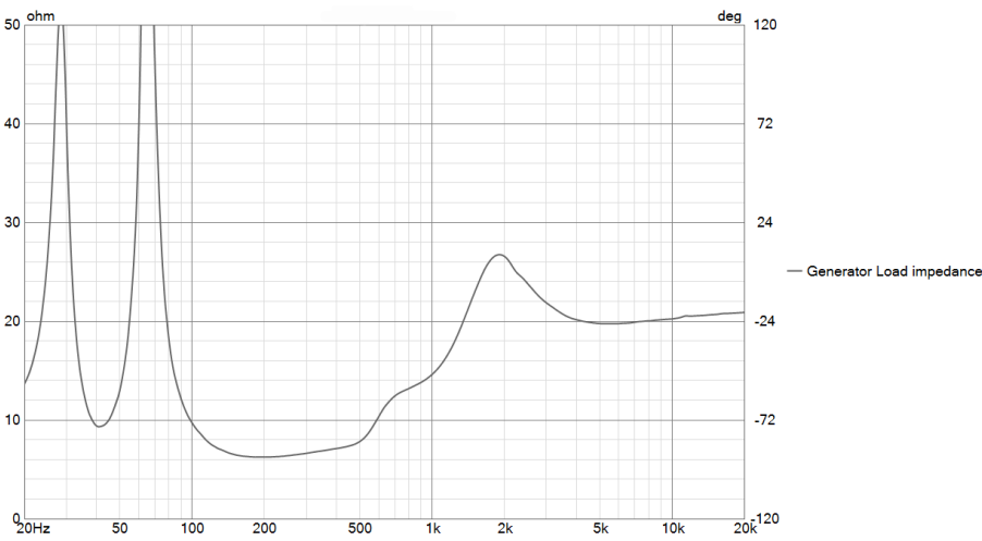
COLLAR IMPEDANCE
