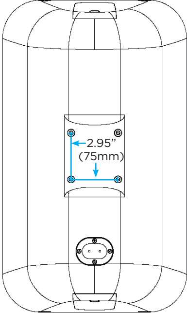
Loudspeaker Back
