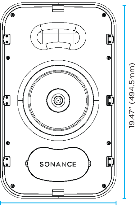
Loudspeaker Front 11.57" (293.9mm)
